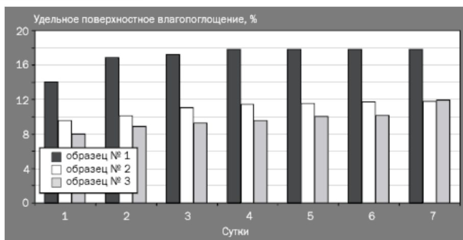
Fig. 2. Specific surface moisture absorption of the encapsulated mass “Celnincil” at various sizes sample surface
