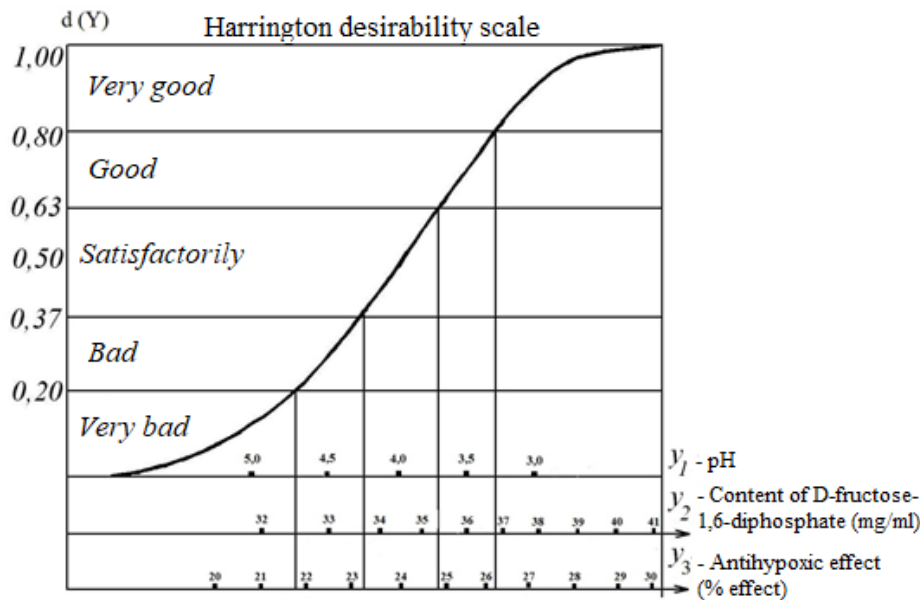
Fig.1. Desirability function scale
